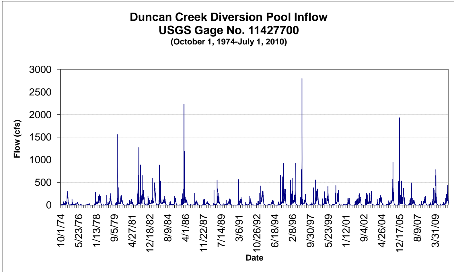
Figure AQ 9-3. Duncan Creek Diversion Pool Historical Inflow.
