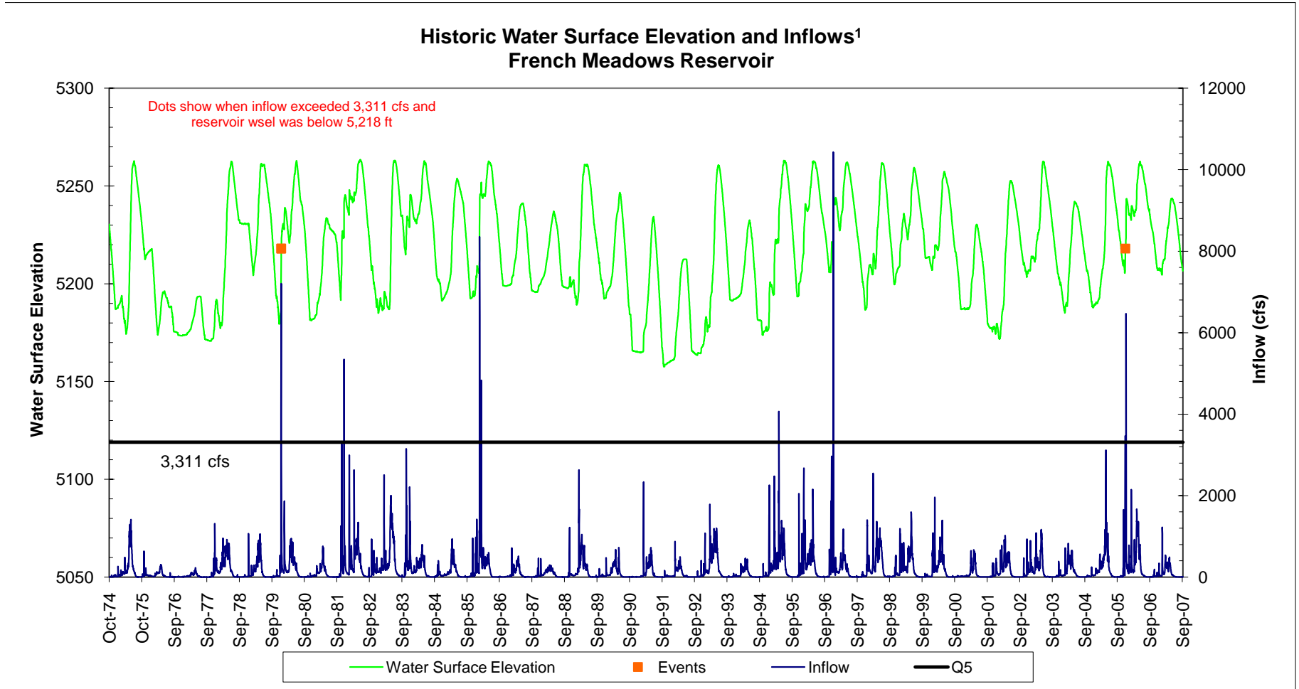
Figure AQ 9-2. Historic Water Surface Elevation and Inflows at French Meadows Reservoir.
