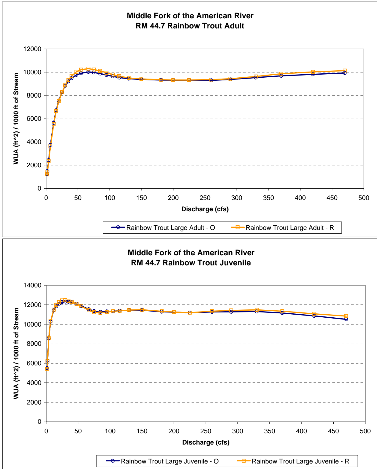
Figure J-3. Middle Fork of the American River - MF44.7 Weighted Usable Area Results by Species/Lifestage from Velocity Modeling Sensitivity Analysis Comparing Original (O) and Revised (R) Modeled Velocities. Negative Velocities Removed from Revised Set.
