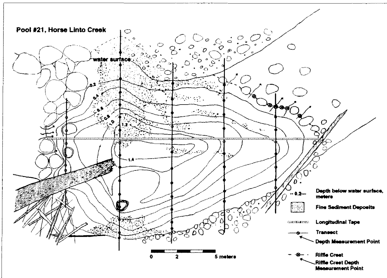
Figure 2—Pool #21, Horse Linto Creek, showing location of the longitudinal tape, transects, measurement points for water and fine sediment depth, the riffle crest, and measurement points for riffle crest depth.
