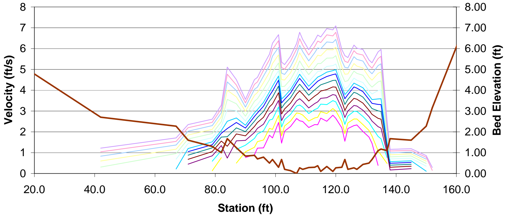
Figure D-8. Mammoth Bar: Modeled Current Velocities
