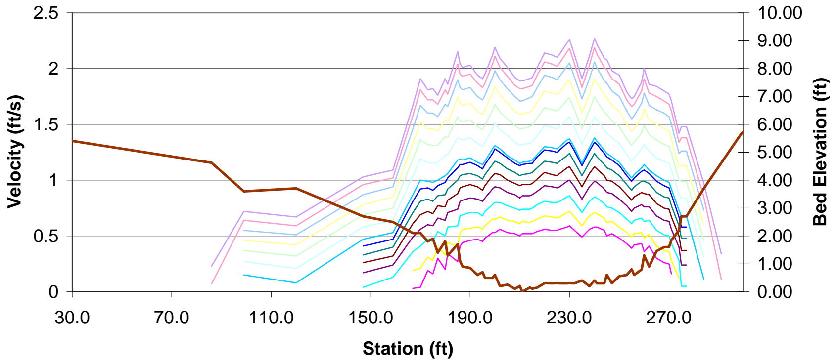
Figure D-6. Poverty Bar: Modeled Current Velocities
