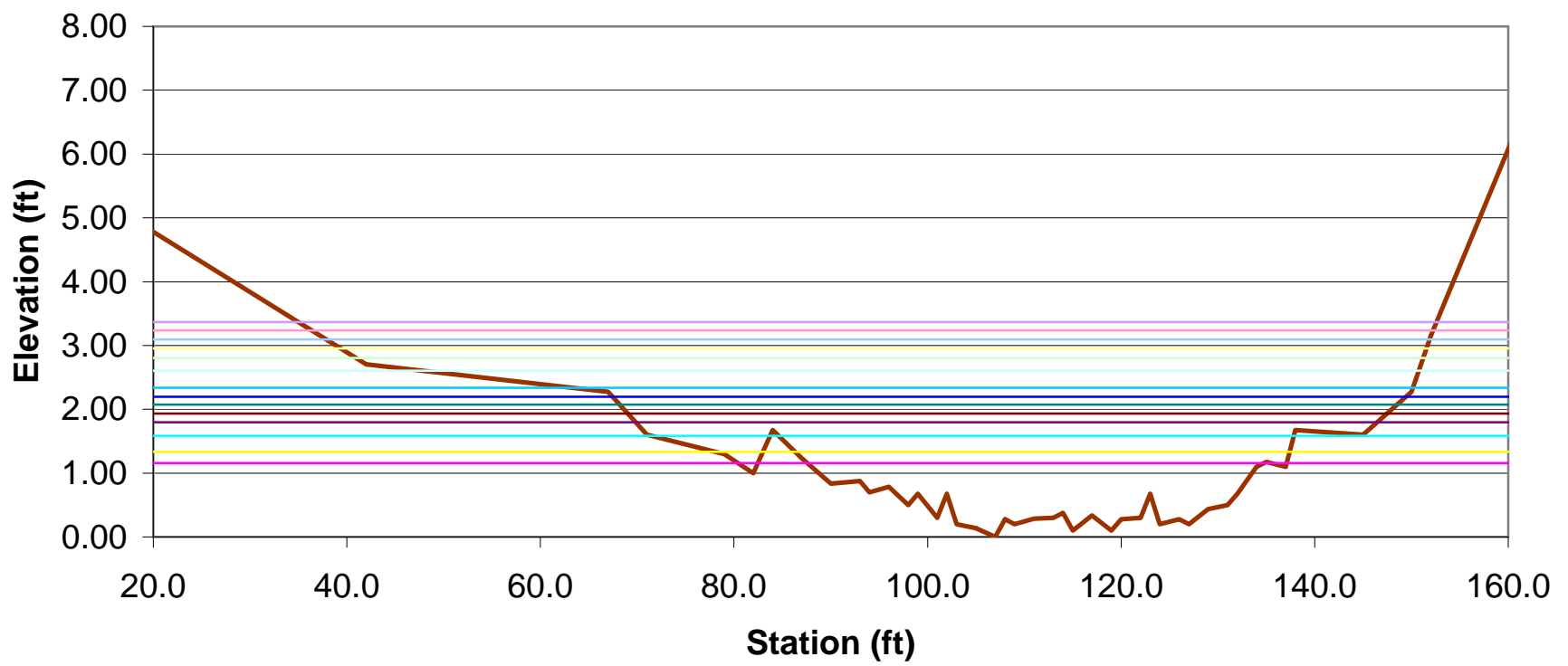
Figure D-7. Mammoth Bar: Modeled Water Surface Elevations
