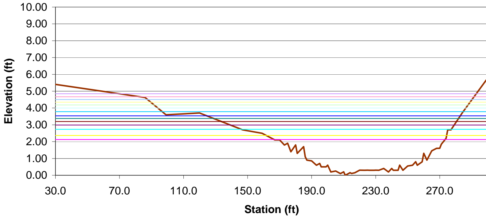
Figure D-5. Poverty Bar: Modeled Water Surface Elevations
