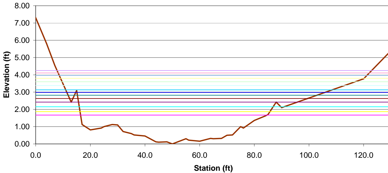
Figure D-9. Coffer Dam: Modeled Water Surface Elevations
