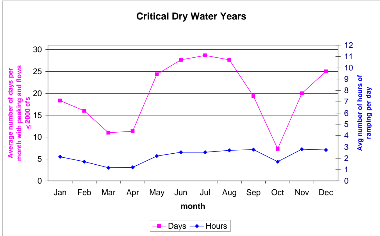
Figure REC 4-27. Average Number of Days and Hours that Ramping Occurred in the Peaking Reach (continued).
