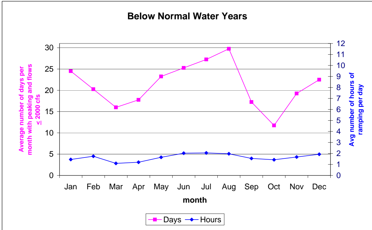
Figure REC 4-27. Average Number of Days and Hours that Ramping Occurred in the Peaking Reach.
