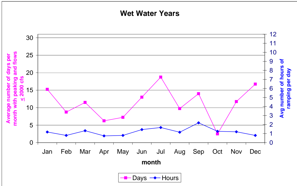
Figure REC 4-27. Average Number of Days and Hours that Ramping Occurred in the Peaking Reach (continued).
