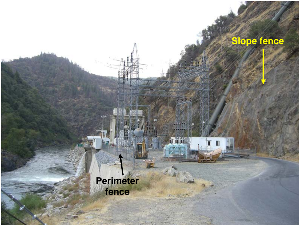
Photo M-2. View of public safety fence (perimeter fence) surrounding Ralston Powerhouse. Also note slope fence along road way. The slope fence is prevents rocks from falling on to the roadway.
